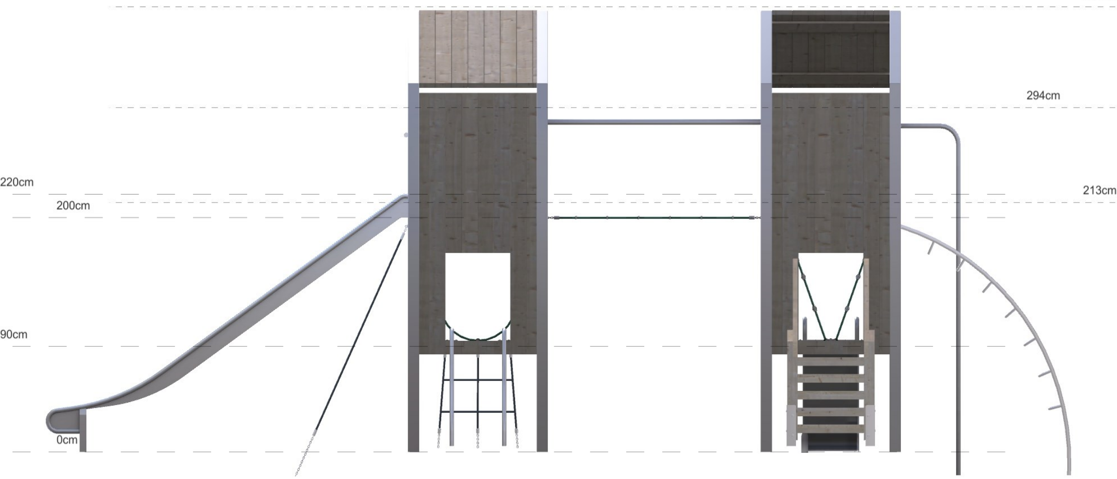
Mounting Heights
